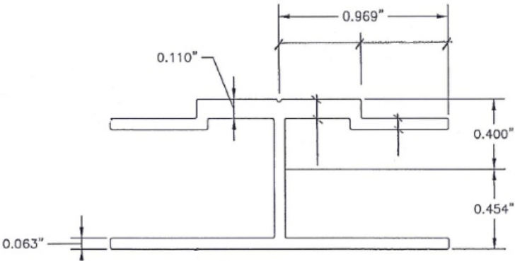
STIFFENER PROFILE
