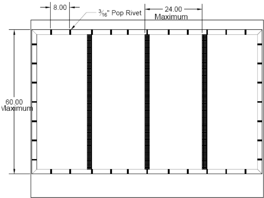
LOCATION OF STIFFENERS ON MCM PANEL
