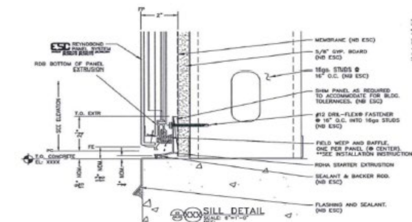
Sill Plate Detail - Route and Return Dry System
