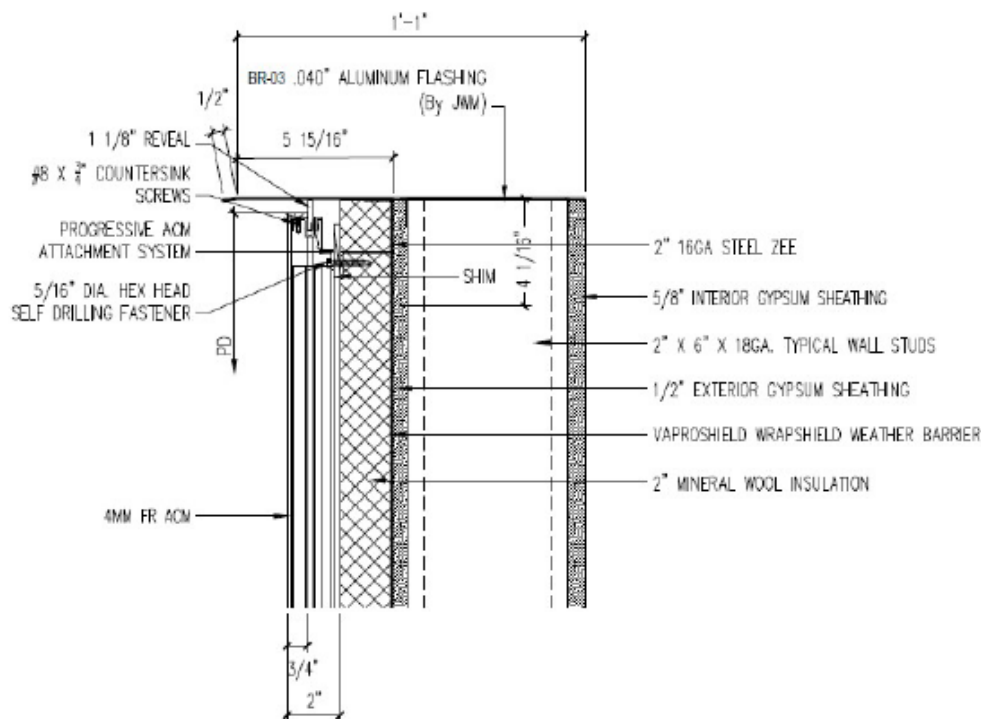
FIGURE 3—WINDOW SILL DETAIL
