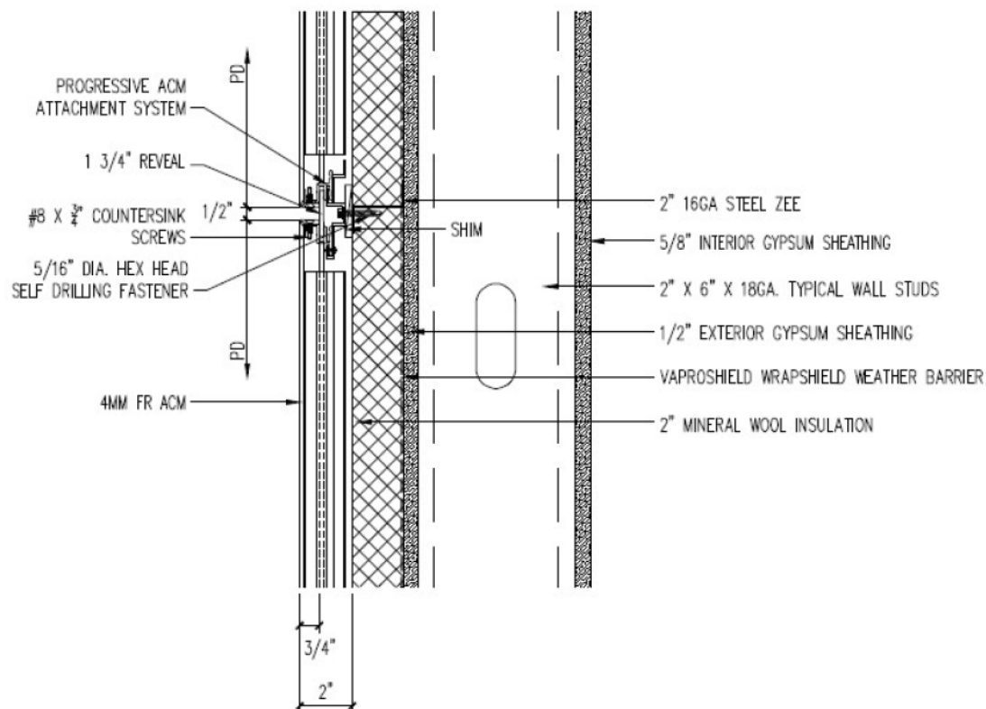
FIGURE 5—HORIZONTAL JOINT DETAIL
