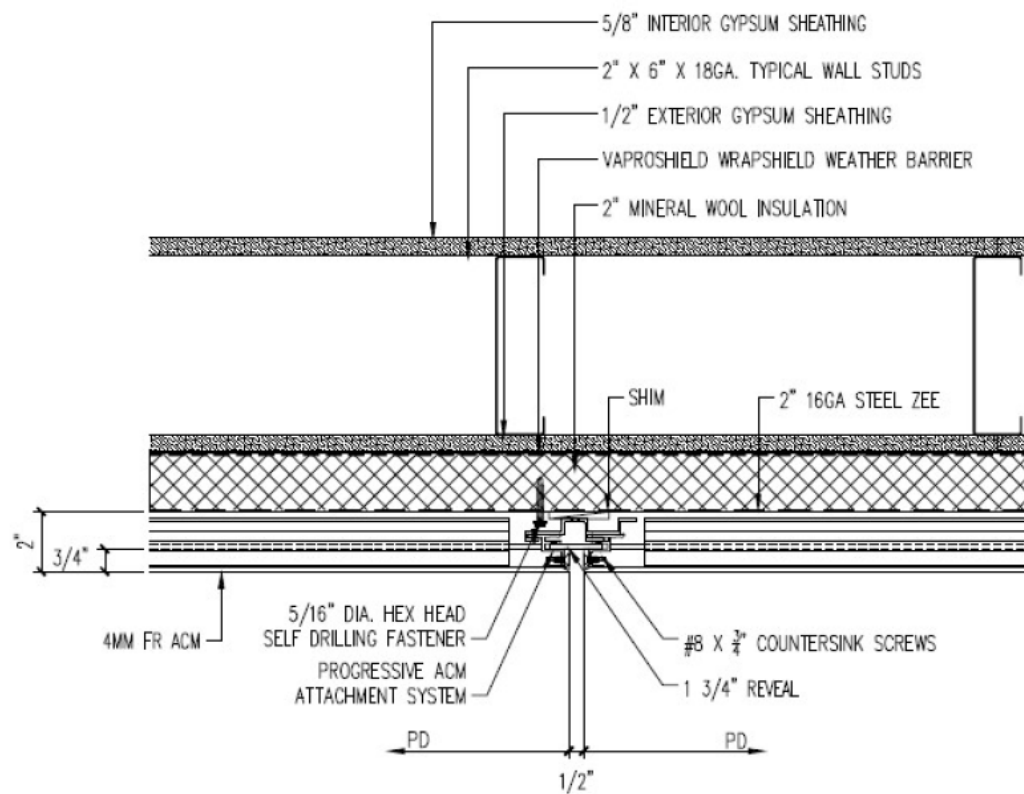
FIGURE 6—VERTICAL JOINT DETAIL
