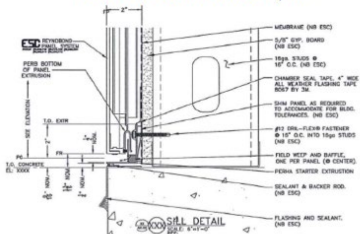
Sill Plate Detail - Route and Return Rain Screen System
