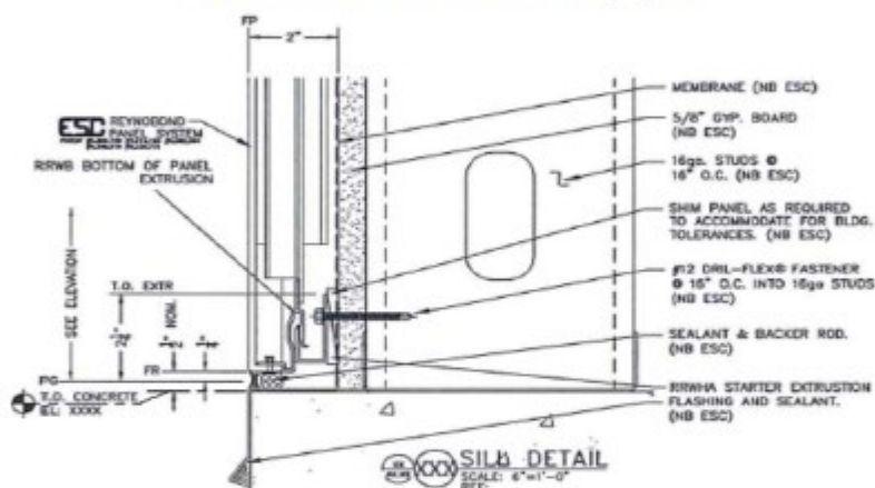
Sill Plate Detail - Route and Return Wet System
